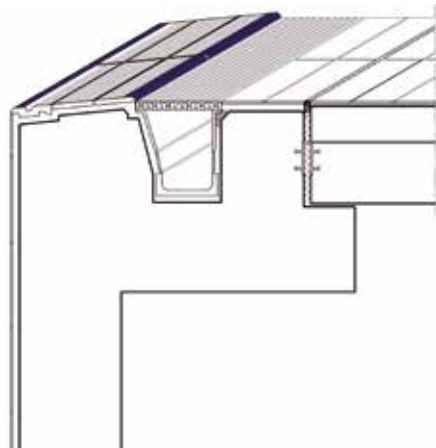
Parallel gratings
