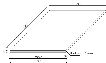
Patio tile with rounded edge on one side
